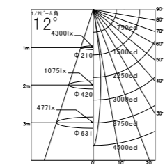
LDR6L-N-E11/D/27/5/12-HC
