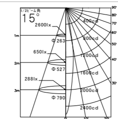
LDR5L-N-E11/D/27/5/15-HC
