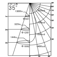
LDR6L-W-E11/D/30/5/35-HC
