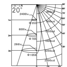
LDR6L-M-E11/D/27/5/20-HC
