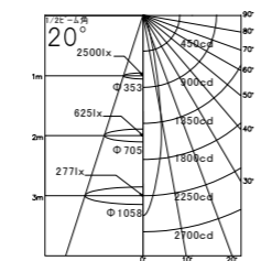
LDR6L-M-E11/D/30/5/20-HC
