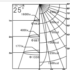
LDR5L-M-E11/D/27/5/25-HC
