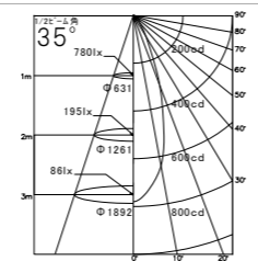
LDR5L-W-E11/D/27/5/35-HC
