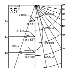
LDR6L-W-E11/D/27/5/35-HC
